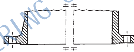
Type 21 Integral flange
